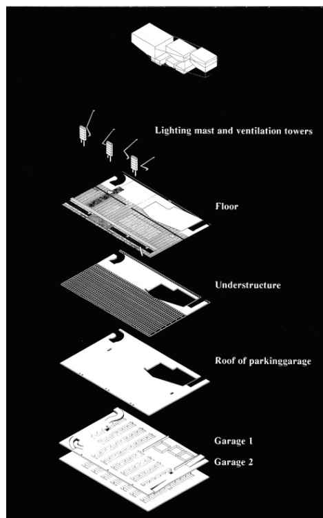
1992_Schouburgplein_West 8
